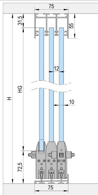
Assembly with surface-mounted track / 3-panel
