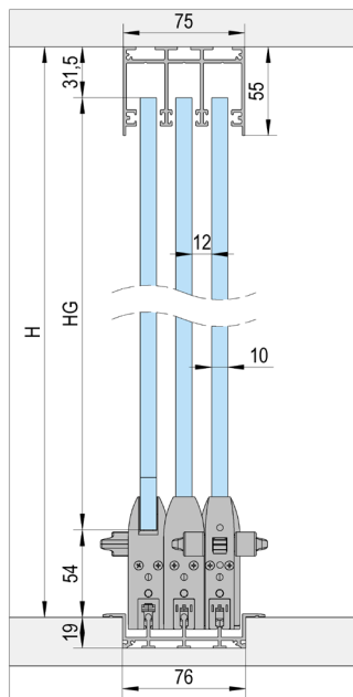
Assembly with recessed track / 3-panel
