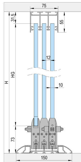
Assembly with recessed track and ramp profiles / 3-panel
